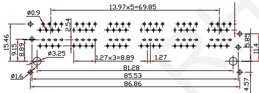
PCB Layout
